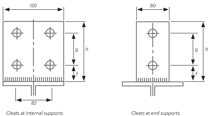
Cleats at internal supports
