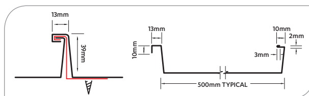
ALL PROFILE DIMENSIONS ARE NOMINAL.
